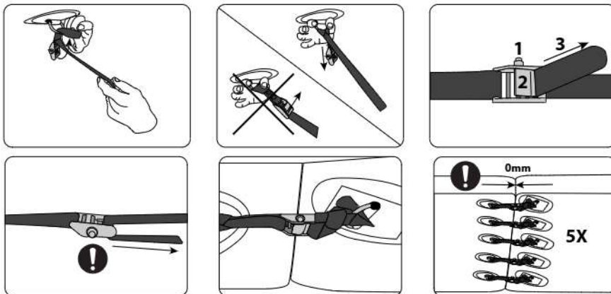
How to connect your Aquaglide Products using the Two-Step Vario-Lock cinch strap
